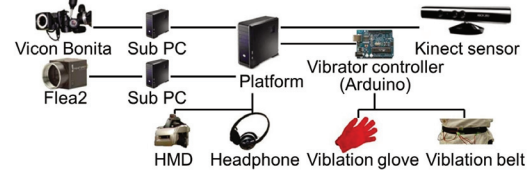
Figure 2. System configuration
